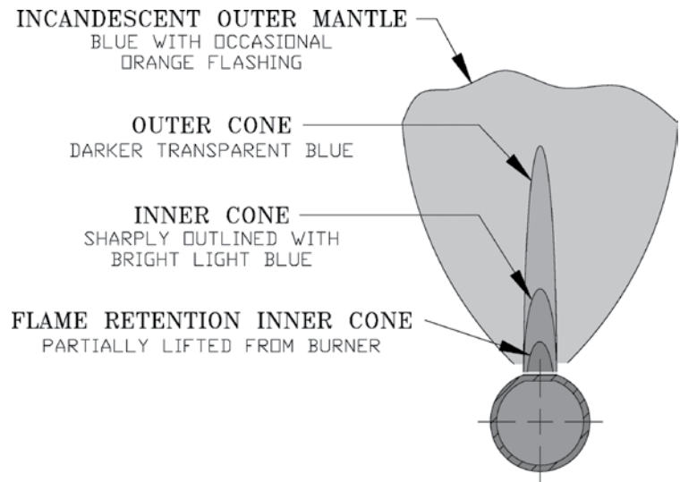
Figure 5: Main Burner Flame
