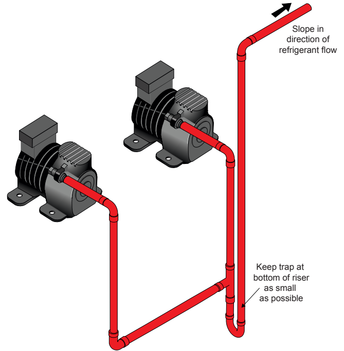
Figure 10: Discharge Line Piping Details
