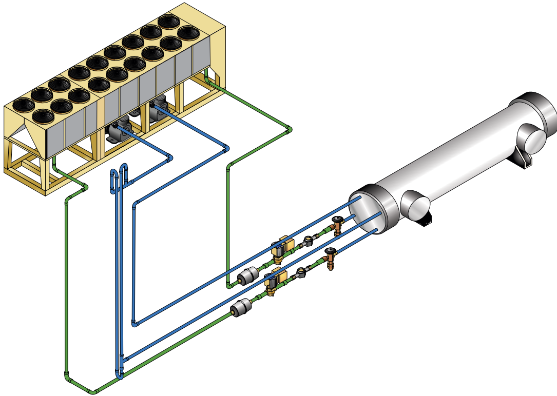
Figure 1: Typical Field Piping Application
