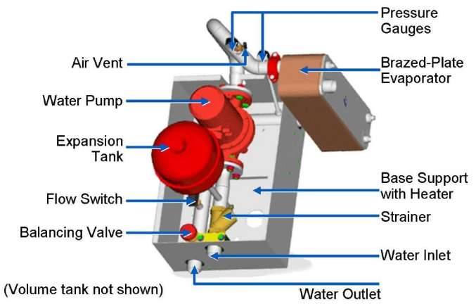
Figure 43 Hydronics Package – Factory-Installed in an Air-Cooled Chiller
