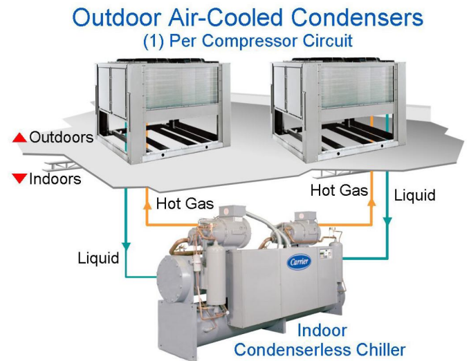
Figure 25 Condenserless Split System Chiller
