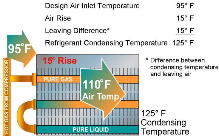
Figure 2 Air-Cooled Condensing Temperature
